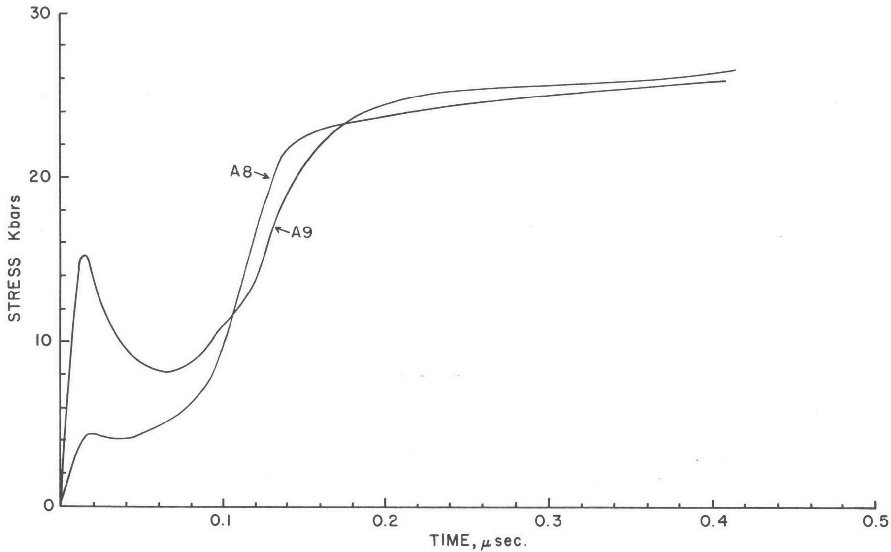
Fig. 27. Stress-time profile for two different specimens of lithium fluoride. The thicknesses of samples A8 and A9 are 2.273 mm and 2.113 mm respectively.
